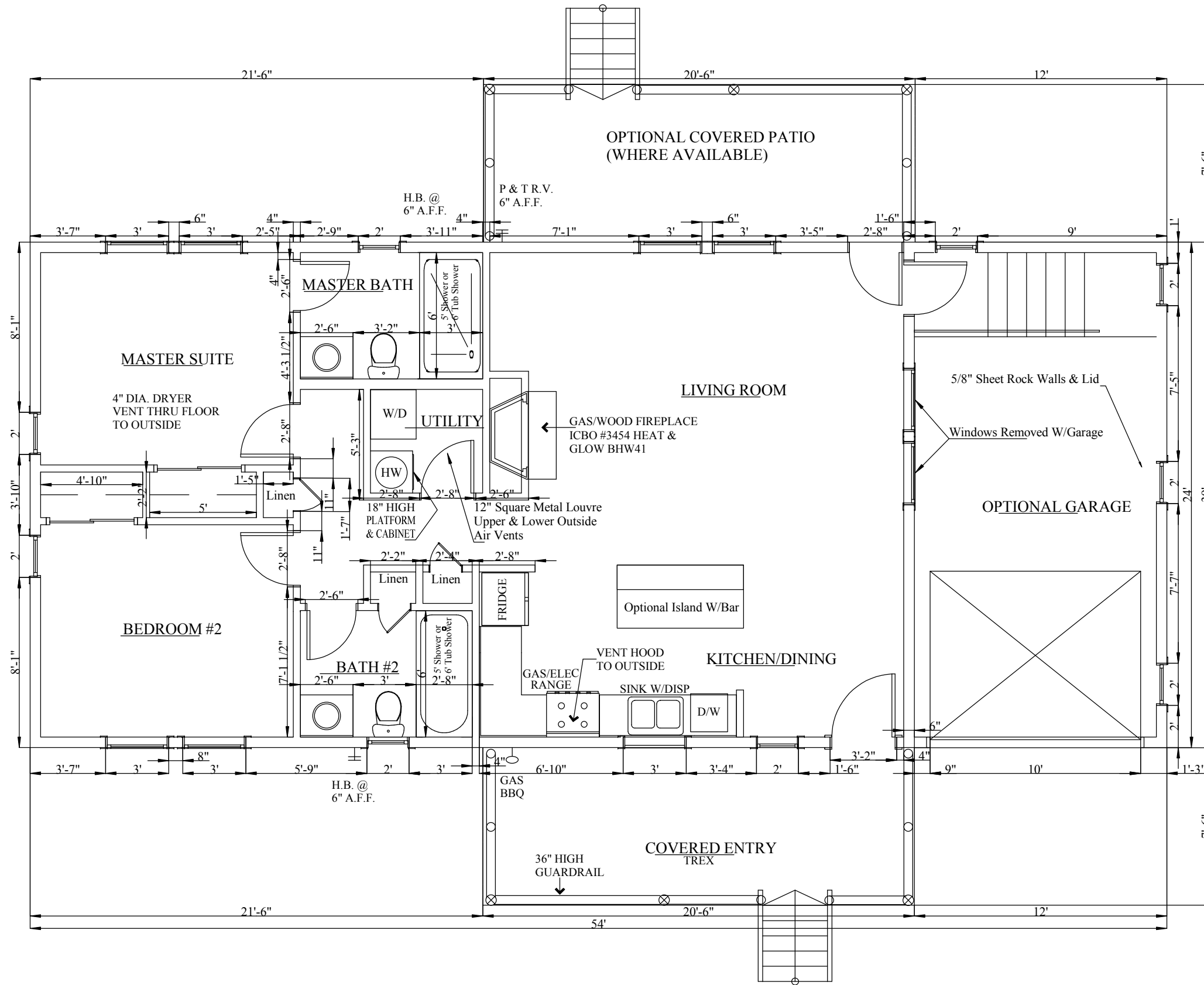
FLOOR PLAN
