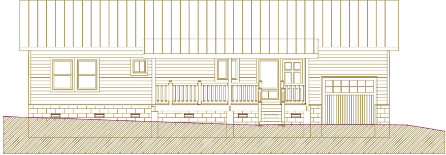
PINE FRONT ELEVATION
