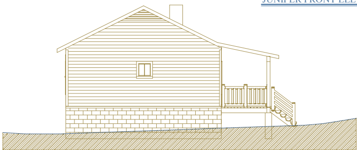
JUNIPER LEFT ELEVATION
