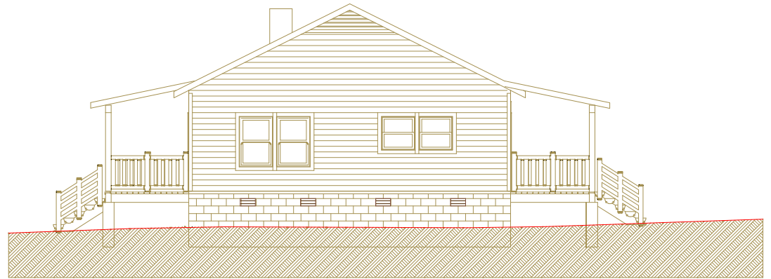
FIR SIDE ELEVATION
