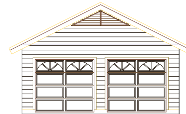
CYPRESS GARAGE ELEVATION
