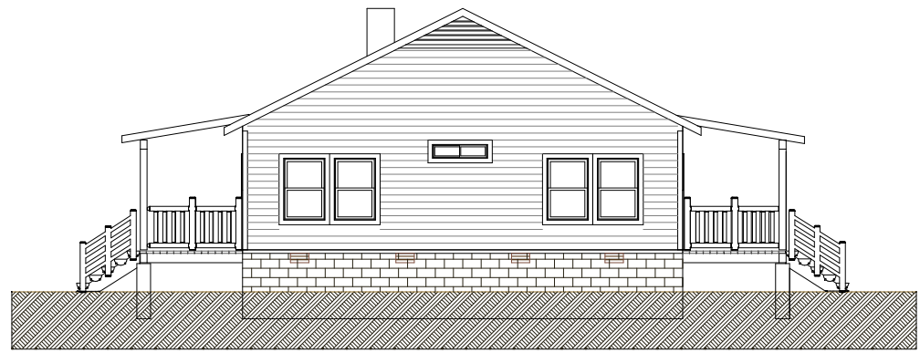
CEDAR LEFT ELEVATION 1/4"=1'-0"
