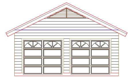
GARAGE ELEVATION PLAN 1/4"=1'-0"
